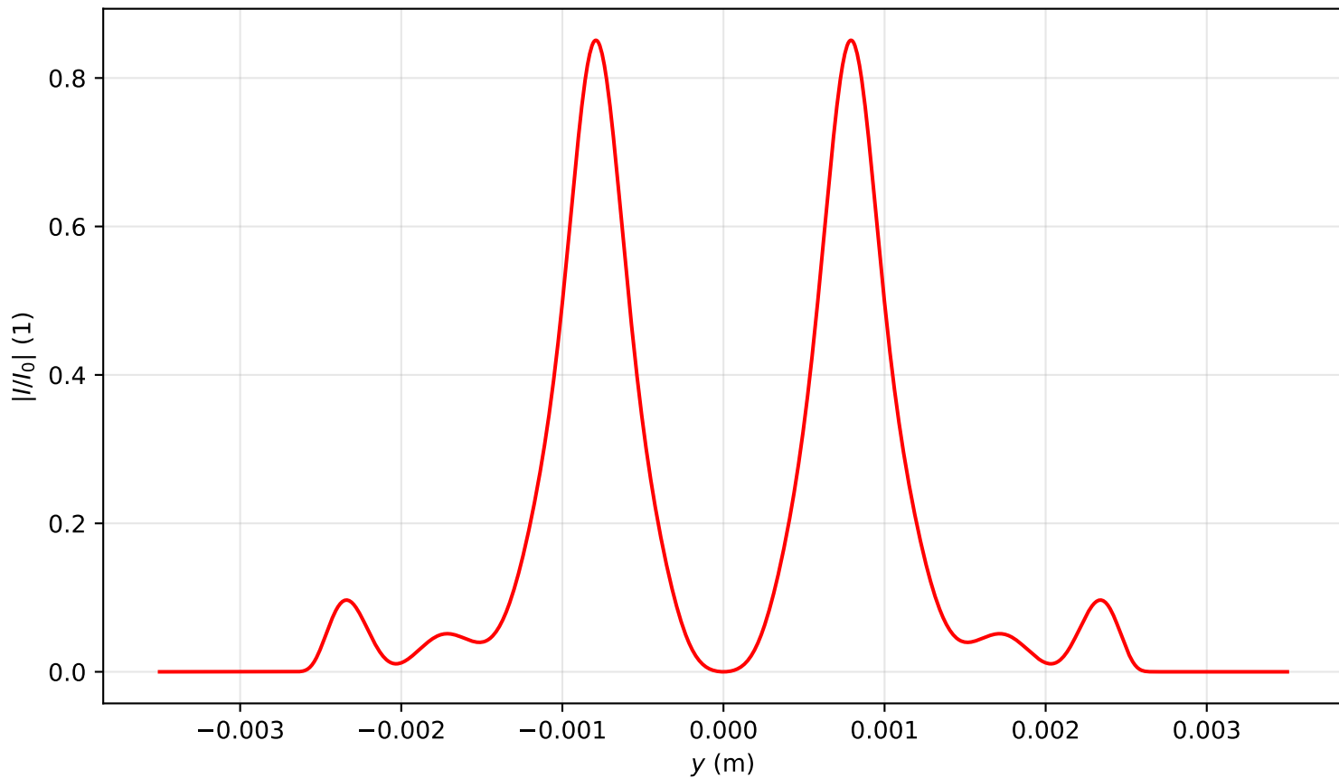
Intensity profile I(x=0, y, z=3.821)/I_0 , P_{in}=5.0P_{cr} , artificial time
